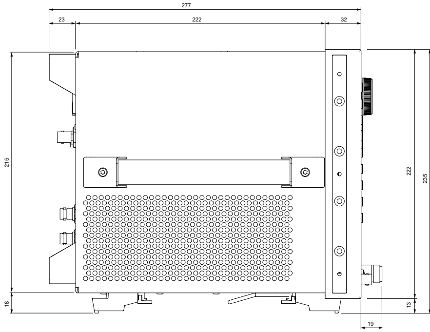
Figure 23. Dimensions (side view, in millimeters)
